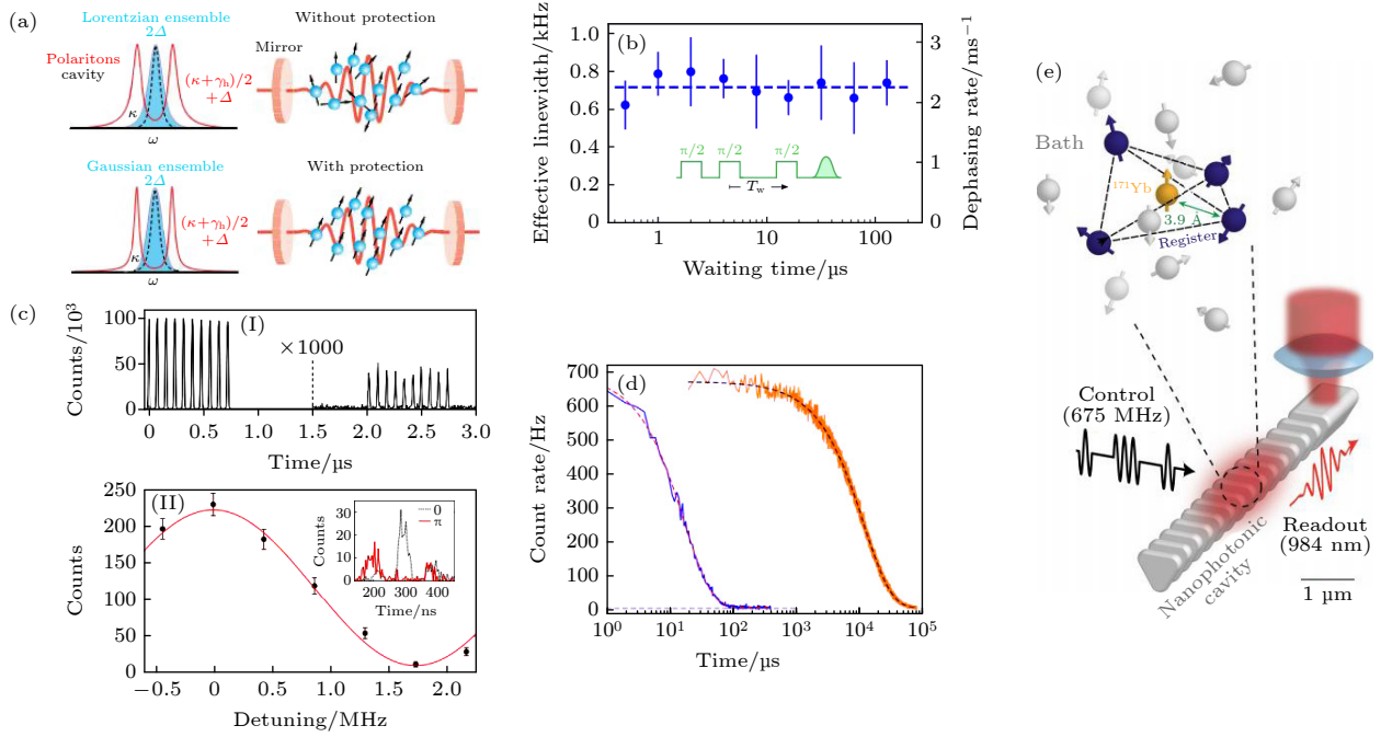
图 11 (a) 腔保护的概念说明: 对于具有洛伦兹线性的系综(上), 由于非均匀展宽的 \Delta , 极化不受保护并发生退相, 即线宽展宽. 而具有高斯线性的系综(下)可以被集体超辐射激发并保护, 不受退相影响. 图中箭头表示每个离子偶极子矢量 [86] . (b) 观察到一个不随等待时间 T_w 变化的有效线宽 \Gamma_{\text{eff}} [110] . 插图为三脉冲光子回波序列. (c) 基于 \text{Er}^{3+} : YSO 光子晶体腔的片上多模量子存储, (I) 存储 10 个时间多模式 2\mu\text{s} ; (II) 通过双梳过程获得的可见度, 插图为在最大建设性干扰(虚线黑线)和最大破坏性干扰(实红色线)情况下的 4 个输出脉冲(中间两个重叠) [87] . (d) 激发脉冲后, 单个腔耦合 \text{Er}^{3+} 离子(蓝色)与没有腔增强的荧光寿命比较(橙色) [72] . (e) 在纳米光子腔中进行光学耦合的 ^{171}\text{Yb} 量子位元的多体核自旋寄存器示意图 [111] . Fig. 11. (a) Conceptual illustration of cavity protection for an ensemble coupled to a cavity mode: For a Lorentzian ensemble (upper), the polaritons are not protected and undergo dephasing (linewidth broadening) due to inhomogeneous broadening \Delta . A Gaussian ensemble (lower) can be fully protected with the collective superradiant excitation free of such dephasing. Arrows represent the phasor of each atomic dipole [86] . (b) A constant effective linewidth \Gamma_{\text{eff}} independent of the waiting time T_w has been observed [110] . Inset: Three-pulse photon echo sequence. (c) On-chip multimode and coherent storage in the \text{Er}^{3+} : YSO nanophotonic cavity. (I) Storage of ten temporal modes for 10\ \mu\text{s} ; (II) visibility curve acquired in a double-comb experiment, and inset is four output pulses (middle two overlapping) in the case of maximally constructive (dashed black line) and maximally destructive (solid red line) interference [87] . (d) Fluorescent lifetime comparison between a single cavity-coupled \text{Er}^{3+} ion (blue) and a bulk ensemble without cavity enhancement (orange) [72] . (e) Schematic of a many-body nuclear spin register for optically coupled ^{171}\text{Yb} qubits in a nanophotonic cavity [111] .
