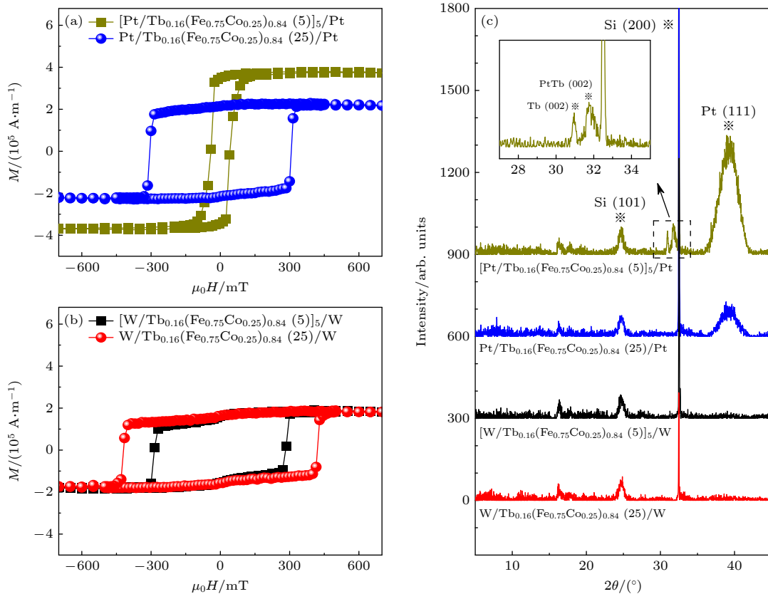
图 4 (a) [Pt(3\text{ nm})/Tb_{0.16}(Fe_{0.75}Co_{0.25})_{0.84}(5\text{ nm})]_5/Pt(3\text{ nm}) 多层膜和 Pt(3\text{ nm})/Tb_{0.16}(Fe_{0.75}Co_{0.25})_{0.84}(25\text{ nm})/Pt(3\text{ nm}) 三层膜的面外方向磁滞回线; (b) [W(5\text{ nm})/Tb_{0.16}(Fe_{0.75}Co_{0.25})_{0.84}(5\text{ nm})]_5/W(5\text{ nm}) 多层膜和 W(5\text{ nm})/Tb_{0.16}(Fe_{0.75}Co_{0.25})_{0.84}(25\text{ nm})/W(5\text{ nm}) 三层膜的面外方向磁滞回线; (c) 上述 Pt, W 多层膜和三层膜样品的 X 射线衍射图, 插图为对应衍射峰的放大图
