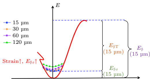
图 9 ( \text{La}_{0.6}\text{Ce}_{0.4}\text{Al}_{10}\text{Co}_{25} 非晶合金激活能随应变演化示意图 Fig. 9. Strain dependence of activation energy for ( \text{La}_{0.6}\text{Ce}_{0.4}\text{Al}_{10}\text{Co}_{25} amorphous alloy.
