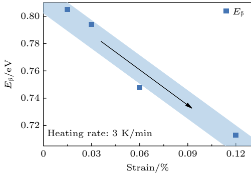
图 8 不同应变下 ( \text{La}_{0.6}\text{Ce}_{0.4}\text{Al}_{10}\text{Co}_{25} 非晶合金的激活能线性拟合结果 Fig. 8. Results of linear fitting of the activation energy of ( \text{La}_{0.6}\text{Ce}_{0.4}\text{Al}_{10}\text{Co}_{25} amorphous alloys with different strain.
