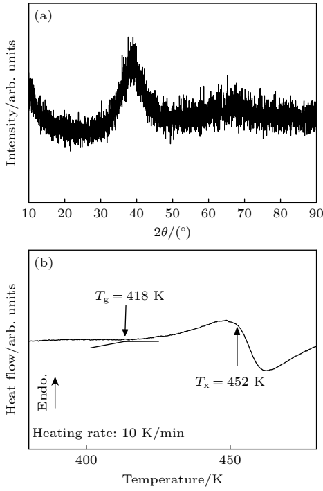
图 1 (a) (La_{0.6}Ce_{0.4})_{65}Al_{10}Co_{25} 非晶合金 X 射线衍射图谱; (b) (La_{0.6}Ce_{0.4})_{65}Al_{10}Co_{25} 非晶合金 DSC 曲线 Fig. 1. (a) XRD pattern of (La_{0.6}Ce_{0.4})_{65}Al_{10}Co_{25} amorphous alloy; (b) DSC curve of (La_{0.6}Ce_{0.4})_{65}Al_{10}Co_{25} amorphous alloy.
