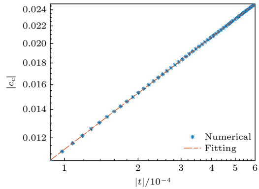
图 7 比热的奇异部分 c_c 随约化温度 t 变化的关系图. 其中蓝色星号表示利用 HOTRG 求得的数值结果, 红色的虚线表示对 (24) 式拟合的结果, 横轴和纵轴采用的都是对数坐标 Fig. 7. Singular part of the capacity c_c as a function of reduced temperature t . Numerical results obtained by HOTRG method are depicted by blue stars, and the red dashed line is a fitting curve for Eq.(24). Both the horizontal coordinate and the vertical coordinate are logarithmic here.
