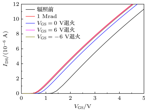
图9 Si-NMOSFET 辐照后不同偏压下的退火效应 Fig. 9. Annealing effect of Si-NMOSFET under different bias voltages after radiation.
