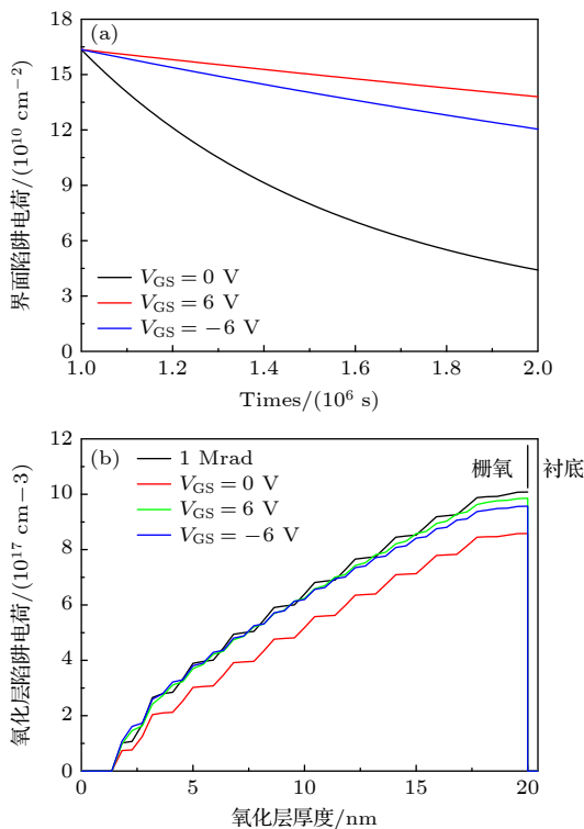
图10 不同偏压下退火后的陷阱电荷 (a) 界面陷阱电荷密度; (b) 氧化层陷阱电荷浓度 Fig. 10. Trapped holes after annealing under the different bias voltages: (a) Trapped interface holes density; (b) trapped holes concentration in oxide layer.
