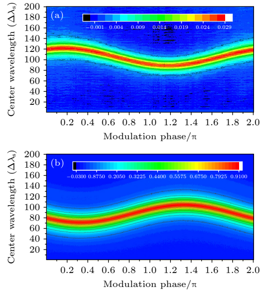
图 6 (a) CO 和 (b) CO 2 波长扫描和调制的激光吸收光谱实验数据对应的 A\varphi 数据矩阵 Fig. 6. Contour image of the data matrix for A\varphi from the laser absorption spectroscopy experiments for (a) CO and (b) CO 2 with the slow scanning and fast modulation of the laser wavelength.
