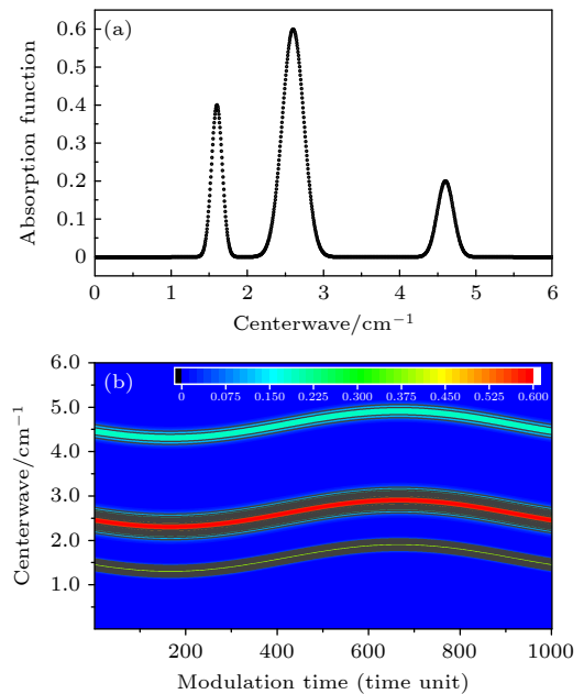
图 1 (a) 3 个吸收谱线的吸收函数; (b) 利用波长的慢速均匀扫描和快速单频正弦调制得到的 A\varphi 数据矩阵等高图像 Fig. 1. (a) Absorption function of three absorption lines; (b) the contour image of the data matrix for A\varphi with a slow uniform scanning of the center wavelength and a fast sinusoidal modulation.
