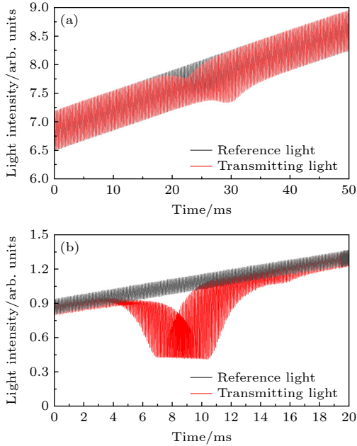
图 5 (a) CO 和 (b) CO 2 波长扫描和调制的激光吸收光谱实验数据 Fig. 5. Tested data of the laser absorption spectroscopy experiments for (a) CO and (b) CO 2 with the slow scanning and fast modulation of the laser wavelength.
