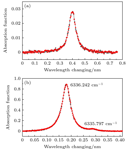
图 7 利用图 6 所示的实验得到的数据矩阵和时间间隔为半个调制周期的两个切片沿波长扫描方向积分值之差的最小绝对值得到的吸收光谱轮廓 (a) CO; (b) CO 2 Fig. 7. Absorption spectrum profiles for (a) CO and (b) CO 2 by minimizing the absolute difference of the integral values along the center wavelength scanning direction between two slices with an interval of half a modulation period and based on the matrix data shown in Fig. 6.
