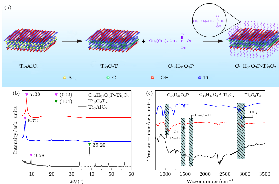
图 1 (a) C_{14}H_{31}O_3P 改性 Ti_3C_2T_x 的过程示意图; Ti_3AlC_2 MAX, Ti_3C_2T_x , C_{14}H_{31}O_3P - Ti_3C_2 的 XRD 衍射图谱 (b) 及红外光谱 (c) Fig. 1. (a) C_{14}H_{31}O_3P modification Ti_3C_2T_x process schematic diagram; XRD diffraction diagram (b) and infrared spectrum (c) of Ti_3AlC_2 MAX, Ti_3C_2T_x , C_{14}H_{31}O_3P - Ti_3C_2 .
