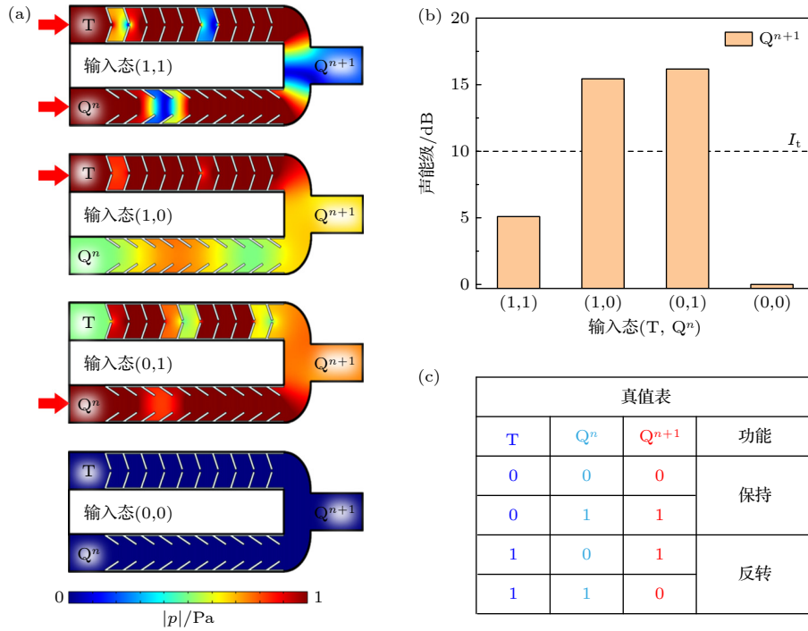
图 2 (a) 数值模拟频率为 3.43 kHz 不同输入态激发 T 触发器产生的声压幅值场分布; (b), (c) 对应的输出端 Q^{n+1} 的声能级和真值表 Fig. 2. (a) Simulated pressure amplitude distributions caused by the T-type trigger with different input states at 3.43 kHz; (b), (c) simulated acoustic intensity levels at the output port Q^{n+1} and truth table.
