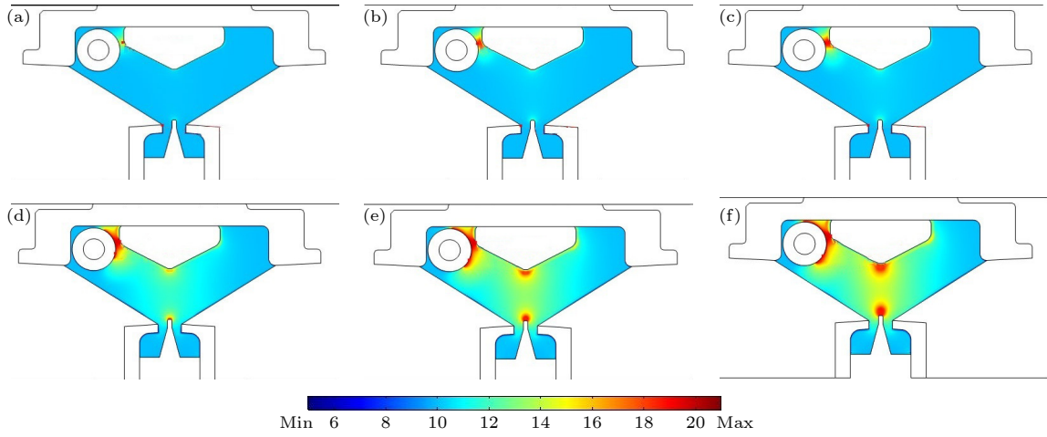
图 6 预电离过程中电子数密度分布情况 (a) t = 25 ns 时, \max = 1.76 \times 10^{15} , \min = 1.37 \times 10^5 ; (b) t = 29 ns 时, \max = 4.40 \times 10^{18} , \min = 9.28 \times 10^4 ; (c) t = 30 ns 时, \max = 2.44 \times 10^{19} , \min = 8.28 \times 10^4 ; (d) t = 35 ns 时, \max = 4.40 \times 10^{18} , \min = 9.28 \times 10^4 ; (e) t = 45 ns 时, \max = 1.50 \times 10^{24} , \min = 1.74 \times 10^{-7} ; (f) t = 47 ns 时, \max = 1.62 \times 10^{24} , \min = 1.88 \times 10^{-7}
