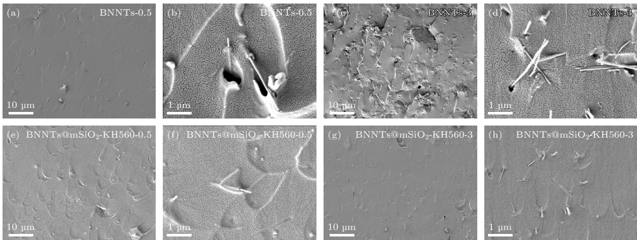
图3 (a)–(d)不同BNNTs含量的复合电介质SEM图像; (e)–(h)不同BNNTs@mSiO 2 -KH560含量的复合电介质SEM图像 Fig. 3. (a)–(d) SEM images of composite dielectric with different BNNTs contents; (e)–(h) SEM images of composite dielectric with different BNNTs@mSiO 2 -KH560 contents.
