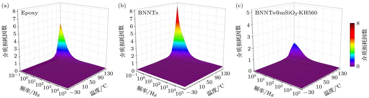
图 6 不同填料复合电介质的介质损耗因数温谱图 Fig. 6. Temperature spectrum of dielectric loss factor of composite dielectric with different fillers.
