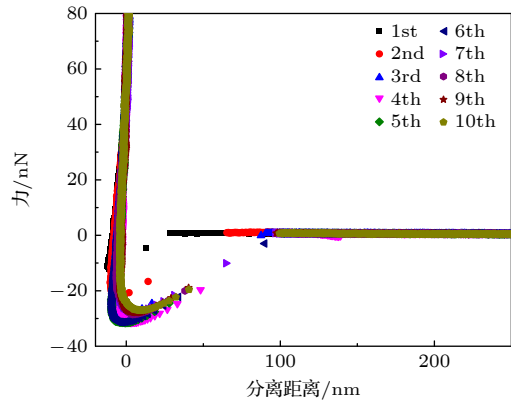
图 10 部分脱气处理条件下, 不同接近次数时疏水颗粒与基板间的相互作用力 Fig. 10. Interaction force between hydrophobic particles and substrate at different approaching times under the condition of partial degassing treatment.
