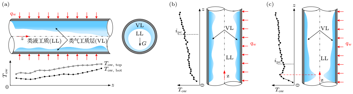
图 8 水平管和垂直向上管流动传热机理图 (a) 水平管; (b) 正常传热模式的垂直向上管; (c) 传热恶化模式的垂直向上管 Fig. 8. Schematics showing the mechanisms for heat transfer and flow characteristics in horizontal and vertical upward tubes: (a) Horizontal tube; (b) vertical upward tube in normal heat transfer mode; (c) vertical upward tube in heat transfer deterioration mode.
