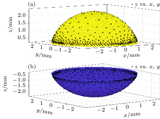
图5 电压最大(260 V)时,双凸液体透镜的液滴面型拟合结果 (a)上界面;(b)下界面 Fig. 5. Droplet profile of the biconvex liquid lens is fitted at maximum voltage (260 V): (a) Upper interface; (b) lower interface.
