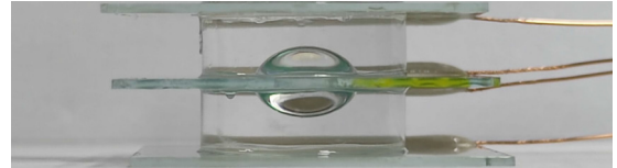
图7 制备的含有圆孔平板电极结构的双凸液体透镜实物图 Fig. 7. Physical image of the biconvex liquid lens with a circular hole plate electrode structure.
