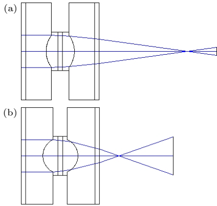
图6 双凸液体透镜的光路图 (a)初始状态(0 V);(b)电压加到最大(260 V) Fig. 6. Optical path diagram of the biconvex liquid lens: (a) Initial state (0 V); (b) maximum voltage state (260 V).
