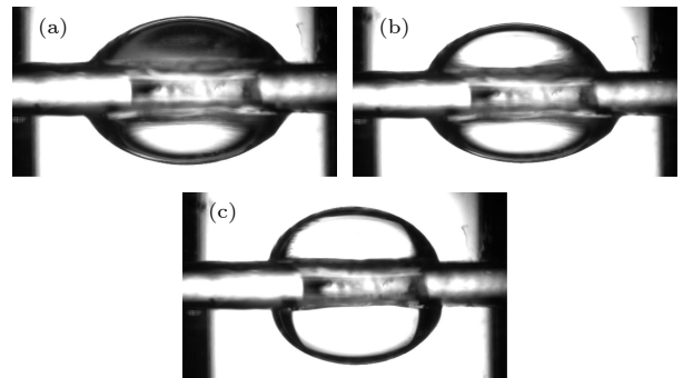
图8 不同电压下的双凸液体透镜面型图 (a)0 V;(b)160 V;(c)260 V Fig. 8. Surface profiles of the biconvex liquid lens under different voltages: (a) 0 V; (b) 160 V; (c) 260 V.
