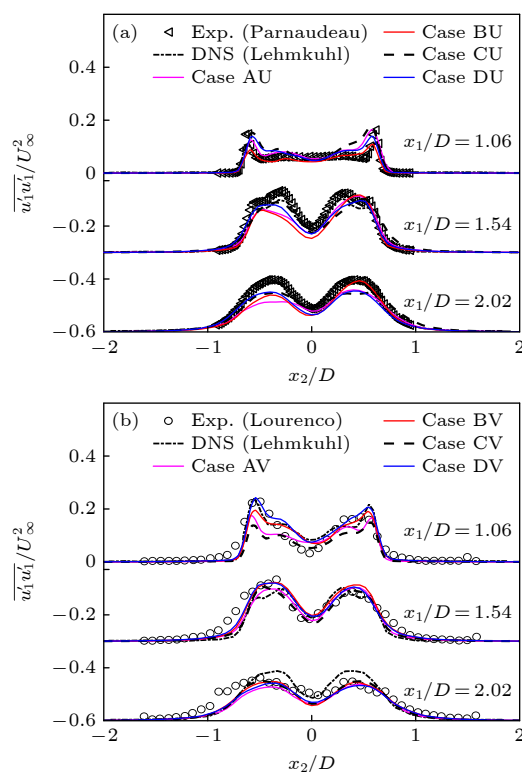
图 8 圆柱后方不同站位处各向同性流向雷诺应力剖面特性 Fig. 8. Distribution characteristics of isotropic stream-wise Reynolds stresses at different locations in the backside of the circular cylinder.
