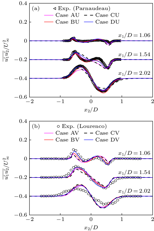
图 10 圆柱后方不同站位处各向异性雷诺应力剖面特性 Fig. 10. Distribution characteristics of anisotropy cross-flow Reynolds stresses at different locations in the backside of the circular cylinder.
