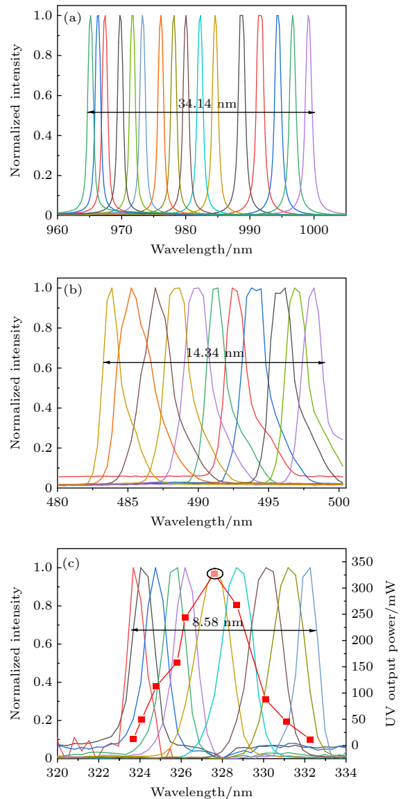
图 5 (a) 基频激光的波长调谐图; (b) 倍频激光的波长调谐图; (c) 紫外激光的波长调谐与输出功率图 Fig. 5. (a) Wavelength tuning of the fundamental laser; (b) wavelength change of the frequency doubled laser; (c) tuning range and powers of the UV output.
