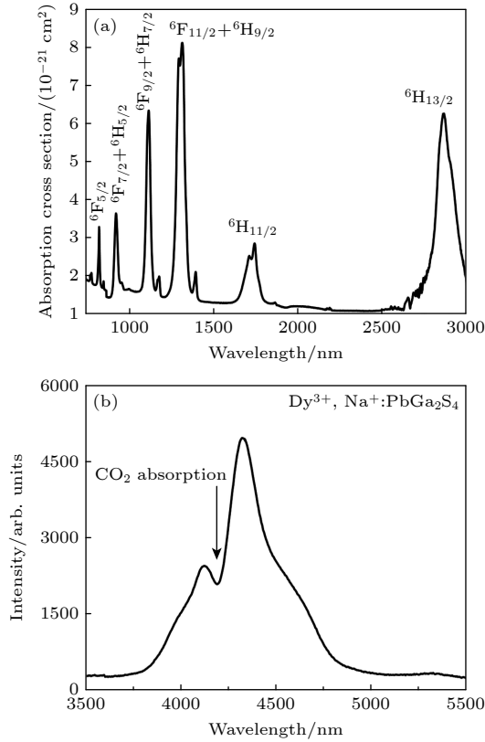
图2 \text{Dy}^{3+} , \text{Na}^{+}:\text{PbGa}_2\text{S}_4 晶体的吸收光谱和荧光发射谱 [26] (a) 500—3000 nm 吸收光谱; (b) 3500—5500 nm 荧光发射谱 Fig. 2. Absorption spectrum and fluorescence emission spectrum of \text{Dy}^{3+} , \text{Na}^{+}:\text{PbGa}_2\text{S}_4 crystal [26] : (a) Absorption spectrum range from 500 to 3000 nm; (b) fluorescence emission spectrum range from 3500 to 5500 nm.
