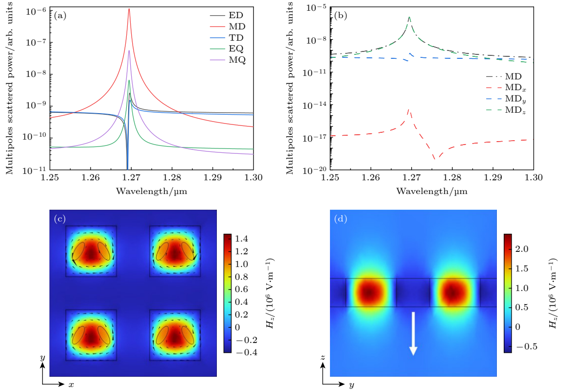
图 3 (a) x 偏振光入射时的多极分解结果, ED, MD, TD, EQ, MQ 分别表示电偶极子、磁偶极子、环偶极子、电四极子、磁四极子; (b) 磁偶极子的散射功率在 x, y, z 方向上的分量; (c) x - y 平面的电磁场分布; (d) y - z 平面的电磁场分布 Fig. 3. (a) Multipole decomposition results during x -polarized normal incidence light, ED, MD, TD, EQ, MQ represent electric dipole, magnetic dipole, toroidal dipole electric, quadrupole and magnetic quadrupole, respectively; (b) x, y and z components of the MD; (c) electromagnetic field distribution in the x - y plane; (d) electromagnetic field distribution in the y - z plane.
