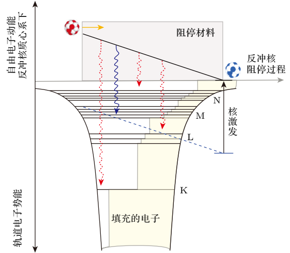
图2 阻停过程中电子俘获致核激发的示意图 Fig. 2. Schematic diagram of nuclear excitation by electron capture in ion-stopping process.
