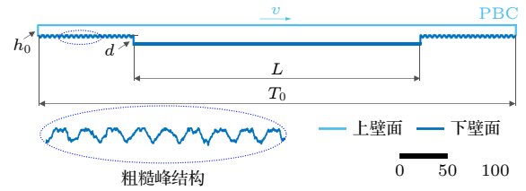
图 1 计入粗糙峰的矩形微观复合织构的润滑模型 Fig. 1. The lubrication model of textured surfaces consisting of rectangular grooves and rough peaks.
