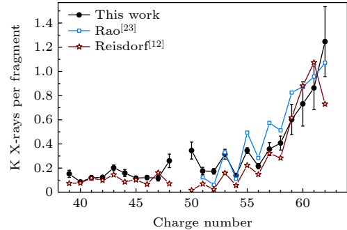
图 9 ^{252}\text{Cf} 自发裂变的平均每碎片 K X 射线产额与电荷数的关系 Fig. 9. Average K X-rays per fragment as a function of nuclear charge for ^{252}\text{Cf} (sf).
