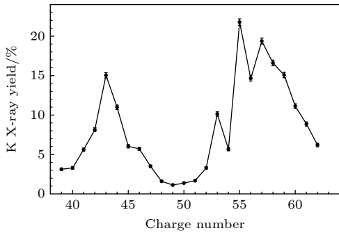
图 8 ^{252}\text{Cf} 自发裂变的 K X 射线相对产额与电荷数的关系 Fig. 8. K X-ray yields of fission fragments as a function of nuclear charge for ^{252}\text{Cf} (sf).
