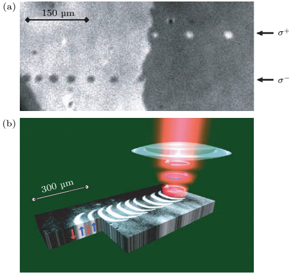
图 4 圆偏振的飞秒激光脉冲全光学磁记录 [6] Fig. 4. All-optical magnetic recording by the circular femto-second laser pulse [6] .
