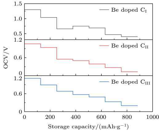
图 13 Be 掺杂石墨双炔的开路电压随储 Li 容量的变化 Fig. 13. Change of open circuit voltage (OCV) of Be doped graphdiyne with storage Li capacity.
