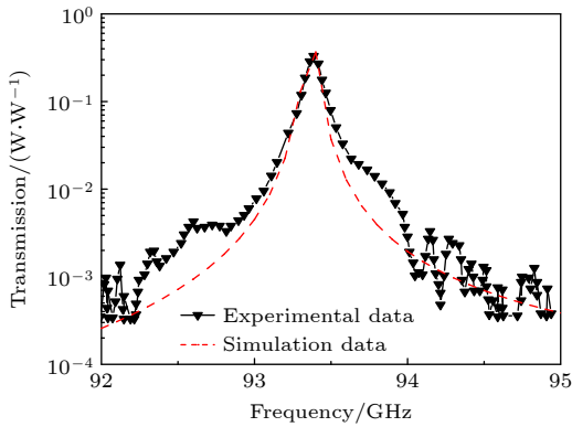
图 2 仿真结果的验证, 实验数据来源于文献 [31] Fig. 2. Verification of simulation results. The experimental data came from the Ref. [31].
