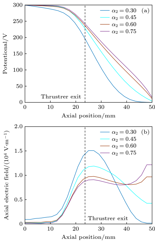
图 5 \alpha_1 = 0.35 时 \alpha_2 对电势 (a) 和电场 (b) 分布的影响 Fig. 5. Influence of \alpha_2 on potential (a) and electric field (b) at \alpha_1 = 0.35 .
