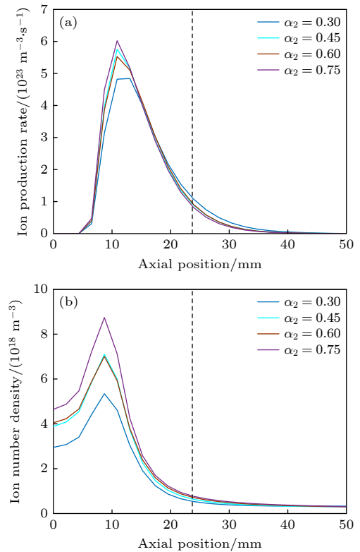
图 6 \alpha_1 = 0.35 时 \alpha_2 对离子产生速率 (a) 和离子密度的影响 (b) Fig. 6. Influence of \alpha_2 on ion production rate (a) and ion number density (b) at \alpha_1 = 0.35 .
