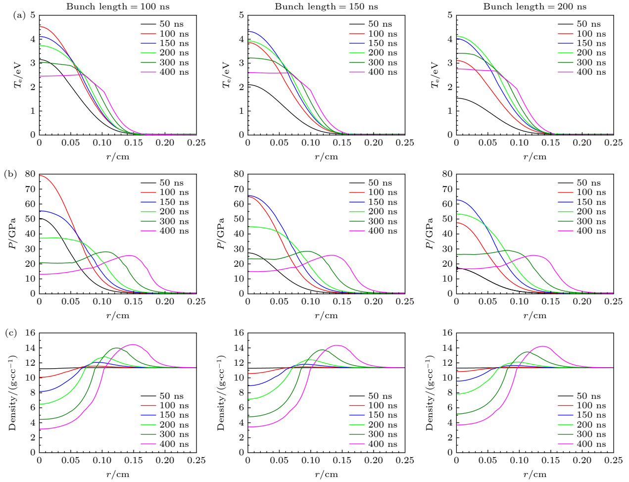
图 5 不同脉冲长度下,束团能量为 500 MeV/u,强度为 1 \times 10^{11} ppp 的物态参数随半径的变化规律 (a) 电子温度; (b) 压强; (c) 密度 Fig. 5. Variation of beam parameters with radius under different bunch lengths, with a beam energy of 500 MeV/u and an intensity of 1 \times 10^{11} ppp: (a) T_e ; (b) P ; (c) density.
