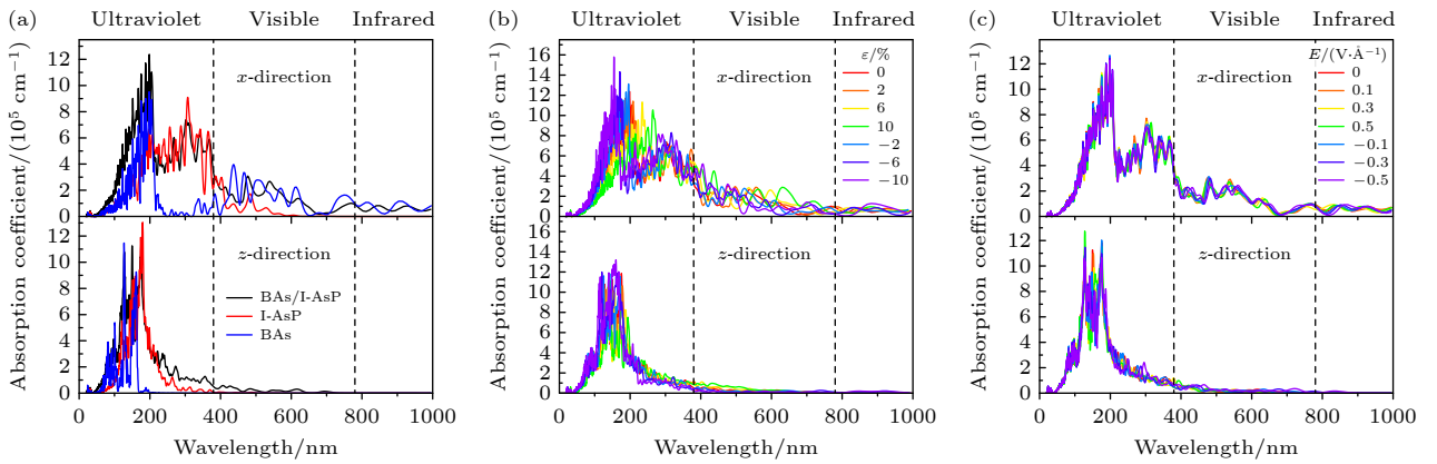
图8 (a) 单层 BAAs、单层 I-AsP 与 BAAs/I-AsP 异质结沿 x 轴和 z 轴的光吸收系数; (b) BAAs/I-AsP 异质结在不同双轴应变下沿 x 轴和 z 轴的光吸收系数变化情况; (c) BAAs/I-AsP 异质结在不同外加电场作用下沿 x 轴和 z 轴的光吸收系数变化情况 Fig. 8. (a) The optical absorption coefficients along the x -axis and z -axis of the monolayer BAAs, I-AsP and the BAAs/I-AsP heterojunction; (b) variations of the optical absorption coefficients along the x -axis and z -axis of the BAAs/I-AsP heterojunction under different biaxial strains; (c) variations of the optical absorption coefficients along the x -axis and z -axis of the BAAs/I-AsP heterojunction under different applied electric fields.
