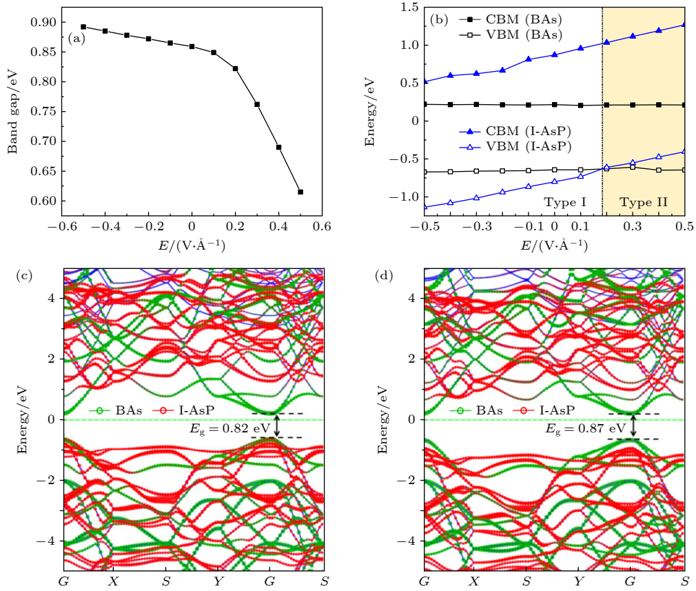
图7 BAAs/I-AsP 异质结构在外加电场下的变化 (a) 带隙变化; (b) 能带边缘变化; (c), (d) E = 0.2 \text{ V}/\text{\AA} 和 -0.2 \text{ V}/\text{\AA} 的能带结构 Fig. 7. Variation of the BAAs/I-AsP heterostructure under an externally applied electric field: (a) Variation of the band gap; (b) variation of the band edges; (c) the energy band structure with E = 0.2 \text{ V}/\text{\AA} and -0.2 \text{ V}/\text{\AA} , respectively.
