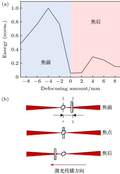
图 3 红外超连续辐射能量随激光离焦量的变化 Fig. 3. Variation of infrared supercontinuum radiation intensity with laser defocus distance.
