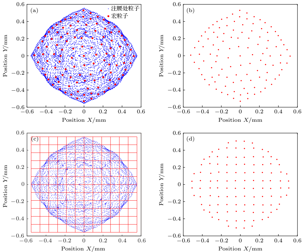
图 7 使用 K 均值聚类算法和网格模型将电子枪注腰处粒子简化为宏粒子 (a) 使用 K 均值聚类算法处理截面粒子; (b) 使用 K 均值聚类算法简化后宏粒子分布; (c) 使用网格模型处理截面粒子; (d) 使用网格模型简化后宏粒子分布 Fig. 7. Particles at the waist of the electron gun are simplified into macroparticles by using the K -means clustering algorithm and the mesh model: (a) The cross-sectional particles are processed by using the K -means clustering algorithm; (b) the distribution of the macro particles after simplification by using the K -means clustering algorithm; (c) the cross-sectional particles are processed by using the mesh model; (d) the distribution of the macro particles after simplification by using the mesh model.
