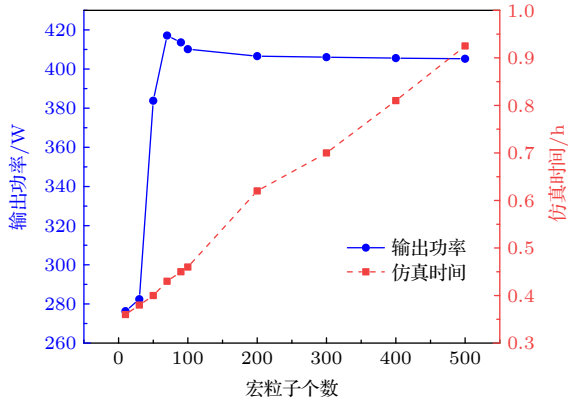
图 6 宏粒子个数与行波管输出功率和仿真时间的关系 Fig. 6. Relationship between the number of macro particles and the output power of the TWT as well as the simulation time.
