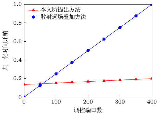
图 3 时间复杂度对比结果 Fig. 3. Comparison results of time complexity.
