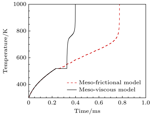
图 9 P = 1 MPa, v = 60 m/s, h_c = 3 \mu m 裂纹中心单元的温度曲线对比图
