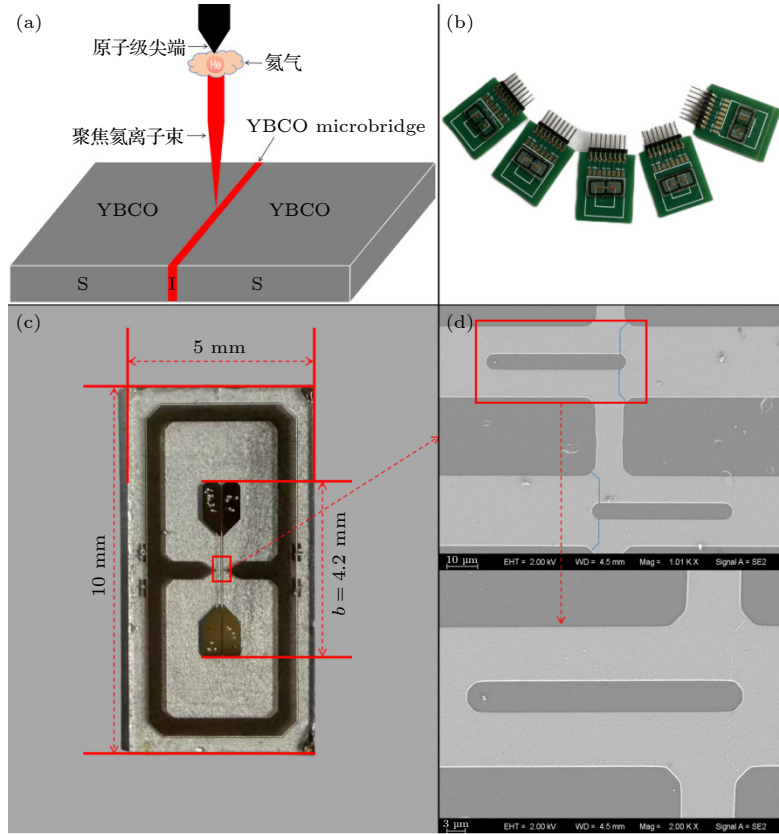
图 1 (a) He-FIB 技术制备约瑟夫森结示意图; (b) 高温超导平面梯度计实物图; (c) 单个梯度计示意图; (d) 梯度计局部放大图 Fig. 1. (a) Schematic of Josephson junction fabrication using He-FIB technology; (b) actual image of high-temperature superconducting planar gradiometer; (c) schematic of a single gradiometer; (d) localized enlargement of the gradiometer.
