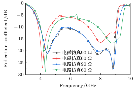
图 12 等效电路的输出结果与电磁仿真结果对比 Fig. 12. Comparison between the results of the equivalent circuit and the electromagnetic simulation.
