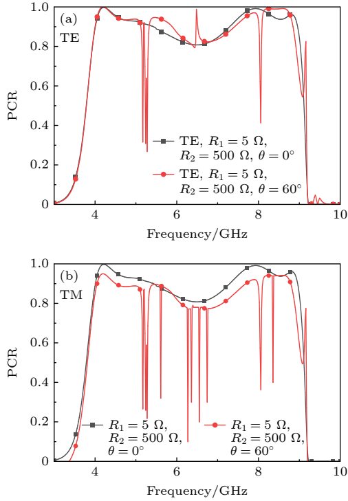
图 9 大入射角下超表面的极化转换率 (a) TE 极化; (b) TM 极化 Fig. 9. Polarization conversion ratio of the metasurface at large incident angles: (a) TE polarization; (b) TM polarization.
