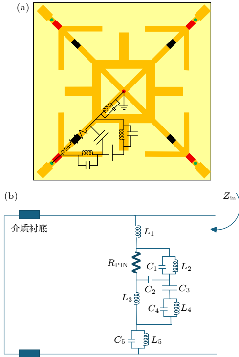
图 11 (a) 顶层与等效电路的对应关系; (b) 等效电路图 Fig. 11. (a) Corresponding relationship between the top layer and the equivalent circuit; (b) equivalent circuit diagram.
