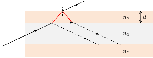
图 1 光从毛细管的空气芯入射至石英包层的几何光路图 Fig. 1. Geometric optical path diagram of light incident from the air core of the capillary to the quartz cladding.
