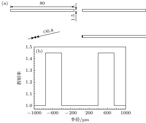
图 6 毛细管结构分析图 (a) CAD 结构图; (b) 折射率分布 Fig. 6. Structural analysis diagrams of the capillary structure: (a) CAD structural diagram; (b) refractive index distribution.
