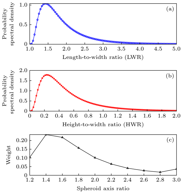
图 3 研究沙尘非球形粒子形态模拟所采用的各类形状分布特征 (a) 三轴椭球体长宽比的概率分布; (b) 三轴椭球体高宽比的概率分布; (c) 旋转椭球体轴长比的权重分布 Fig. 3. Characteristics of the shape distributions adopted for simulating the morphology of non-spherical dust particles: (a) Probability distribution of the length-to-width ratio for tri-axial ellipsoids; (b) probability distribution of the height-to-width ratio for tri-axial ellipsoids; (c) weight distribution of the axial ratio for spheroids.
