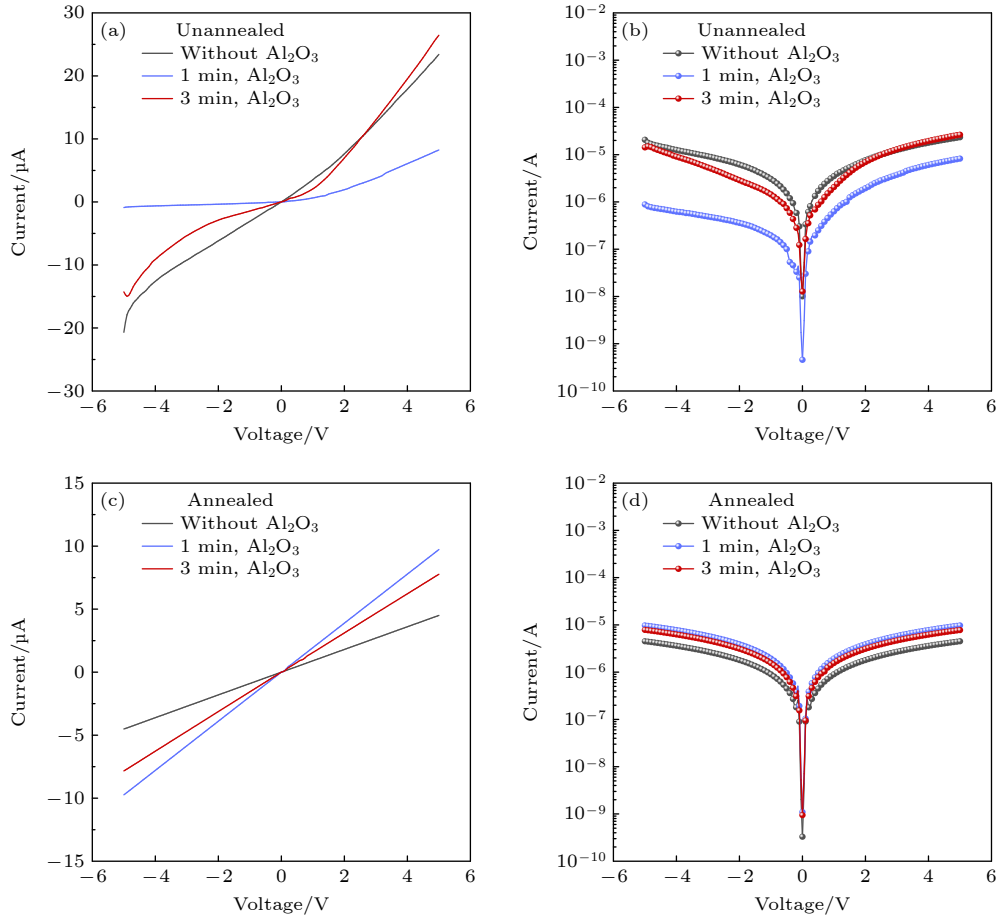
图4 CuO/Al 2 O 3 /ZnO 器件的暗态 I - V 特性 (线性坐标与半对数坐标) (a), (b) 未退火; (c), (d) Ar 氛围下 180 °C 退火 2 h Fig. 4. Dark I - V characteristics of CuO/Al 2 O 3 /ZnO devices (linear and semi logarithmic coordinates): (a), (b) Unannealed; (c), (d) annealed at 180 °C for 2 h in Ar atmosphere.
