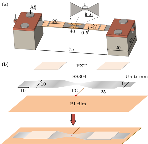
图 2 沸腾实验装置的结构 (a) 实验装置; (b) 加热器的结构 Fig. 2. Structure of the boiling experimental setup: (a) Experimental setup; (b) structure of the heater.
