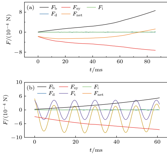
图 10 气泡脱离力平衡模型 (a) f = 0 \text{ Hz} ; (b) f = 100 \text{ Hz} Fig. 10. Bubble detachment force balance model: (a) f = 0 \text{ Hz} ; (b) f = 100 \text{ Hz} .
