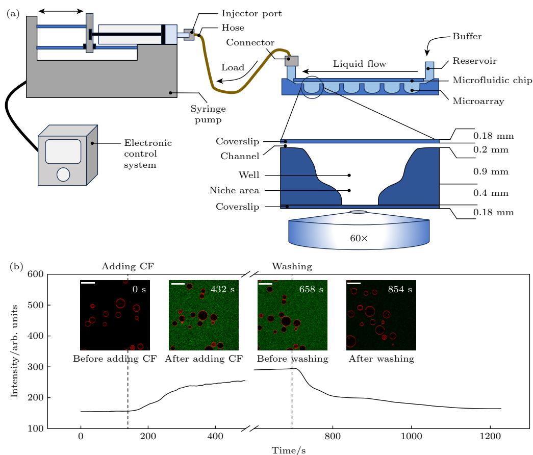
图2 微流控芯片实现无扰换液示意图 (a) 芯片结构与实验设备示意图; (b) 灌注换液过程中的环境荧光强度变化及囊泡共聚焦图像 Fig. 2. Schematic diagram of the microfluidic chip for non-perturbative solution exchange: (a) Schematic diagram of the chip structure and experimental setup; (b) environmental fluorescence intensity variation and confocal images of vesicles during perfusion-based solution exchange.
