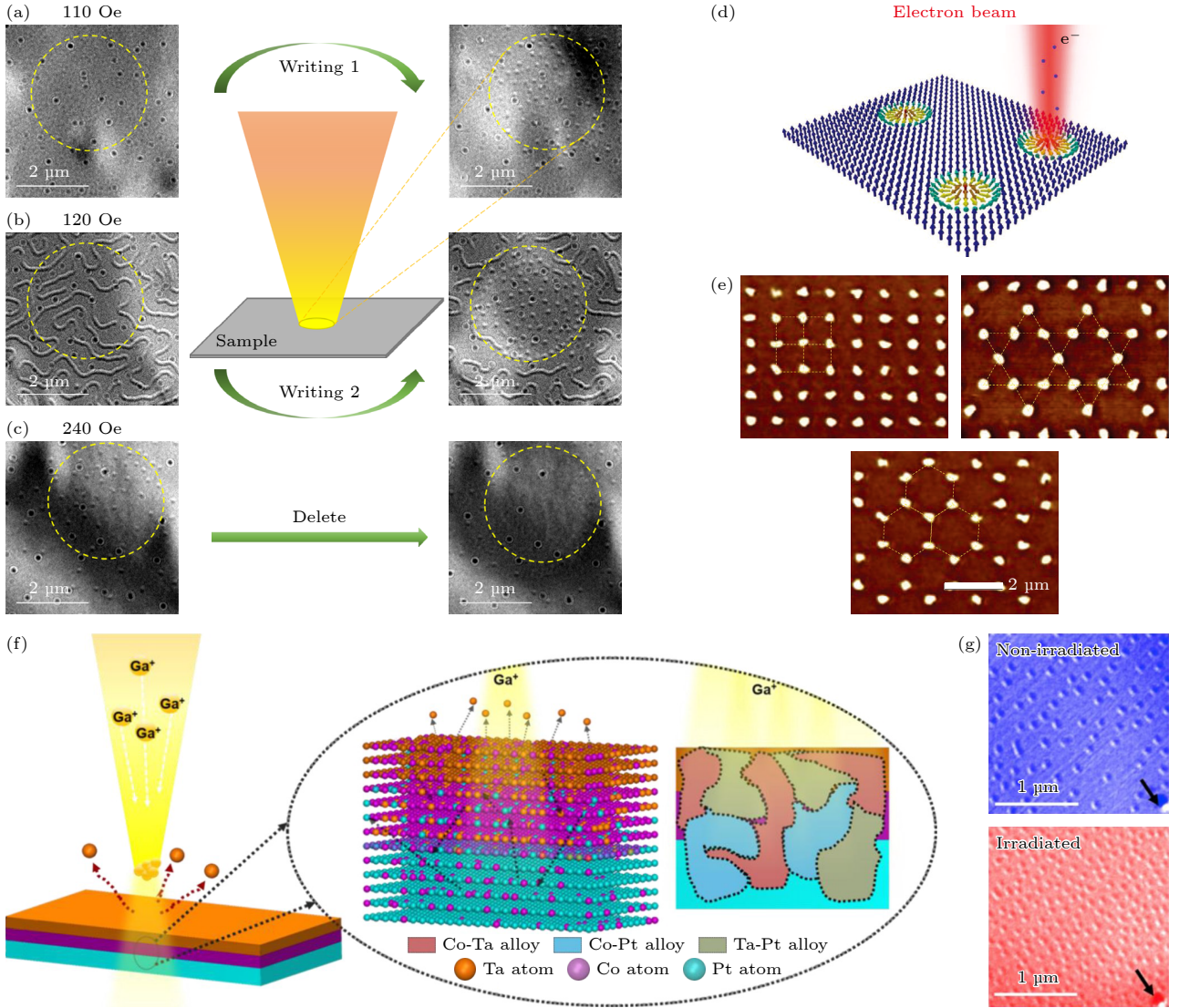
图3 电子束或离子束写入磁斯格明子 (a) 利用聚焦电子束从饱和态写入斯格明子 [58] ; (b) 利用聚焦电子束从迷宫畴态写入斯格明子 [58] ; (c) 利用聚焦电子束擦除斯格明子, 作用区域由黄色虚线圆圈标注, 比例尺为 2 μm, 需注意, 图像中高对比度环绕的黑点为杂质点在欠焦模式下产生的菲涅耳条纹 [58] ; (d) 利用电子束产生斯格明子的示意图 [59] ; (e) 电子束光刻制备的方形、kagome 型及蜂窝构型人工斯格明子晶格的 MFM 图像, 黄色虚线标示出斯格明子晶格的结构, 单个斯格明子的生成光照时长为 250 ms [59] ; (f) \text{Ga}^+ 辐照单一 Pt/Co/Ta 周期性结构的原理示意图, 原子会沿离子辐照方向及反方向发生迁移, 最终形成合金与晶界 [60] ; (g) 同一位置分别在有/无 \text{Ga}^+ 辐照下采集的洛伦兹透射电镜图像, 其中右下角箭头标注出由镓离子束刻蚀形成的同一孔洞, 用作定位基准 [60] 。 Fig. 3. Writing magnetic skyrmions by electron beam or ion beam: (a) Writing skyrmions from the saturated state using a focused electron beam [58] ; (b) writing skyrmions from the labyrinth domain state using a focused electron beam [58] ; (c) erasing skyrmions using a focused electron beam, with the affected region marked by a yellow dashed circle and a scale bar of 2 μm, note that the black dots surrounded by high contrast fringes are Fresnel fringes generated by impurity particles in the underfocus mode [58] ; (d) schematic diagram of skyrmion generation by an electron beam [59] ; (e) MFM images of square, kagome, and honeycomb artificial skyrmion lattices fabricated by electron beam lithography, with the lattice structures outlined by yellow dashed lines. The illumination time for writing a single skyrmion is 250 ms [59] ; (f) schematic of \text{Ga}^+ irradiation of a single Pt/Co/Ta periodic structure, where atoms migrate along and opposite to the ion irradiation direction, ultimately forming alloys and grain boundaries [60] ; (g) Lorentz transmission electron microscopy images acquired at the same location with and without \text{Ga}^+ irradiation, where the same hole created by gallium ion beam etching is indicated by an arrow in the lower right corner and serves as a positioning reference [60] .
