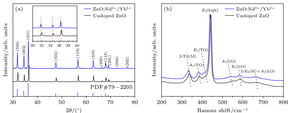
图 1 未掺杂的 ZnO 和 ZnO:Nd 3+ /Yb 3+ 花状分级微米结构 (a) XRD 图谱, 插图为 (100), (002) 和 (101) 峰的放大图; (b) Raman 光谱 Fig. 1. (a) XRD spectra of undoped ZnO and ZnO:Nd 3+ /Yb 3+ flower-like hierarchical microstructures; the inset shows enlarged images of the (100), (002), and (101) peaks; (b) Raman spectra.
