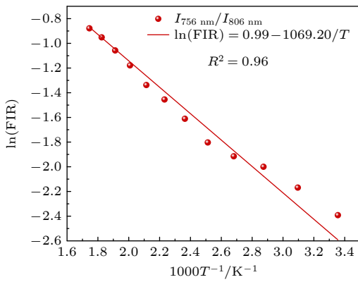
图 9 \ln(\text{FIR}(I_{756 \text{ nm}}/I_{806 \text{ nm}})) 与绝对温度倒数的依赖性关系 Fig. 9. The dependence relationship between \ln(\text{FIR}(I_{756 \text{ nm}}/I_{806 \text{ nm}})) and the reciprocal of the absolute temperature.
