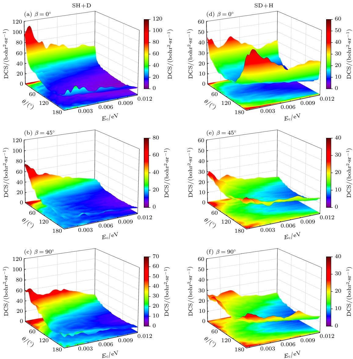
图 4 不同初始 HD 取向, S(^1D) + HD 反应的总 DCS 随散射角与碰撞能的变化关系 (a)–(c) 属于 SH 通道; (d)–(f) 属于 SD 通道 Fig. 4. Total DCS as a function of scattering angle and collision energy for the S(^1D) + HD reaction under different initial HD orientations: (a)–(c) Correspond to the SH channel; (d)–(f) correspond to the SD channel.
