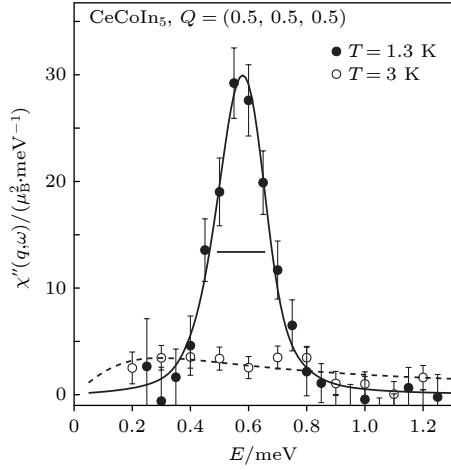
图2 CeCoIn 5 超导态 ( T = 1.3 K) 与正常态 ( T = 3 K) 在 Q_{AF} = (0.5, 0.5, 0.5) 处的非弹性中子散射谱 [30] Fig. 2. Inelastic neutron scattering spectra of CeCoIn 5 at Q_{AF} = (0.5, 0.5, 0.5) in the superconducting state ( T = 1.3 K) and in the normal state ( T = 3 K) [30] .
