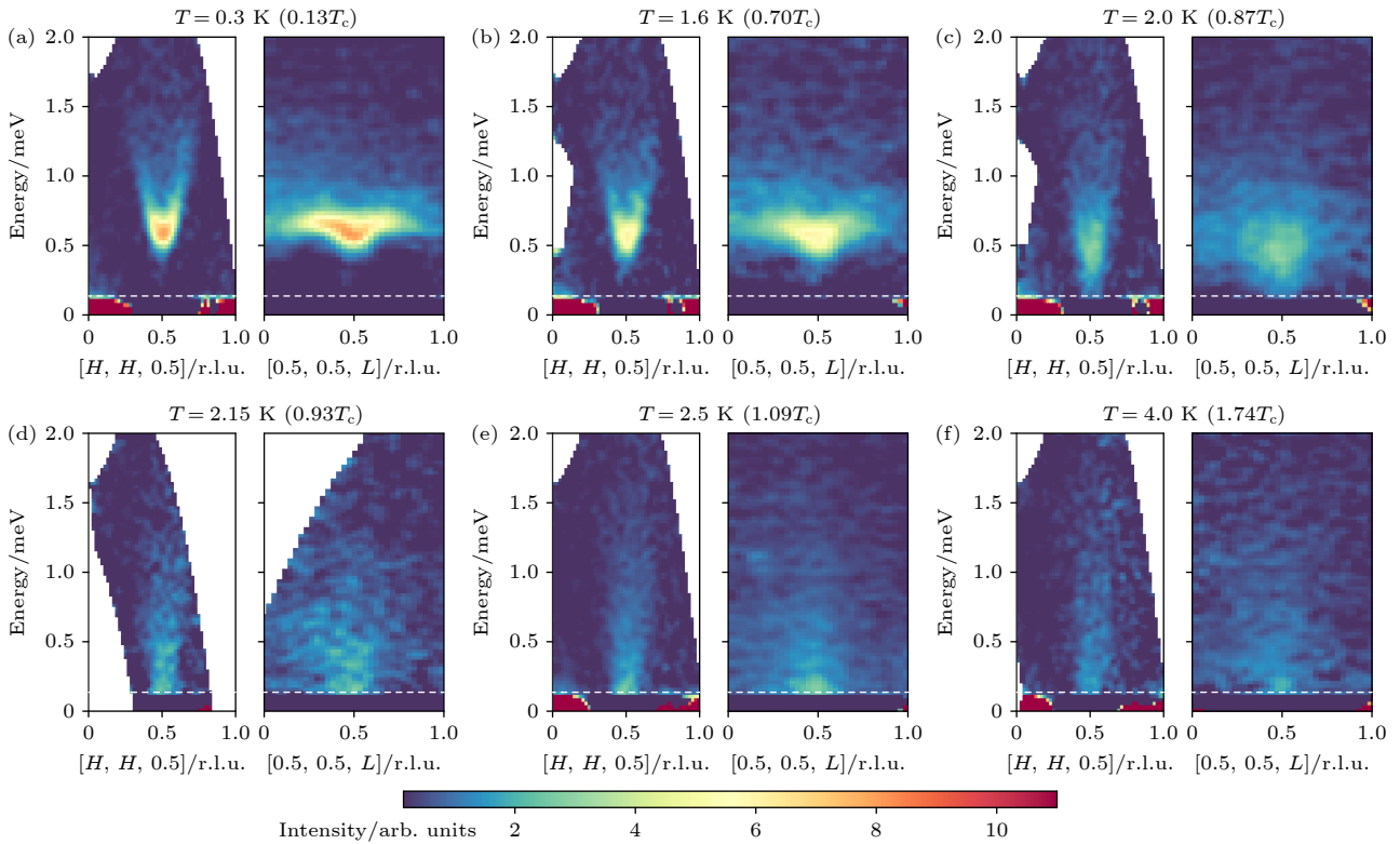
图 7 CeCoIn 5 磁激发谱随温度的演化 [43] (a) T = 0.3 K ( 0.13T_c ); (b) 1.6 K ( 0.70T_c ); (c) 2.0 K ( 0.87T_c ); (d) 2.15 K ( 0.93T_c ); (e) 2.5 K ( 1.09T_c ); (f) 4 K ( 1.74T_c )
