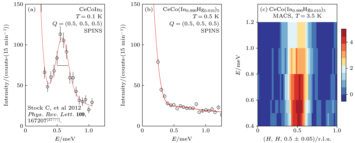
图 12 Q_{AF} = (1/2, 1/2, 1/2) 处的非弹性中子散射对比 [28] (a) CeCoIn 5 在 T = 0.1 K 的超导态自旋共振模 ( E_r \approx 0.55 meV); (b) CeCo(In 0.99 Hg 0.01 ) 5 在 T = 0.5 K 没有显著的磁涨落; (c) CeCo(In 0.99 Hg 0.01 ) 5 在 3.5 K 时沿着 (H, H, 1/2) 的散射强度分布 Fig. 12. Comparison of inelastic neutron scattering at Q_{AF} = (1/2, 1/2, 1/2) [28] : (a) Spin resonance mode of CeCoIn 5 in the superconducting state at T = 0.1 K ( E_r \approx 0.55 meV); (b) absence of significant magnetic fluctuations in CeCo(In 0.99 Hg 0.01 ) 5 at T = 0.5 K; (c) scattering intensity distribution along (H, H, 1/2) in CeCo(In 0.99 Hg 0.01 ) 5 at 3.5 K.
