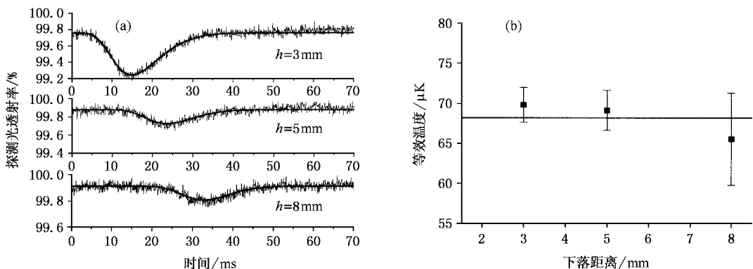
图 3 (a) 将探测光分别置于 h = 3 \text{mm}, 5 \text{mm}, 8 \text{mm} 处测得的短程 TOF 吸收谱 (b) h = 3 \text{mm}, T = 70 \pm 2 \mu\text{K}; h = 5 \text{mm}, T = 69 \pm 3 \mu\text{K}; h = 8 \text{mm}, T = 65 \pm 6 \mu\text{K} ; 平均值约为 68 \mu\text{K}
