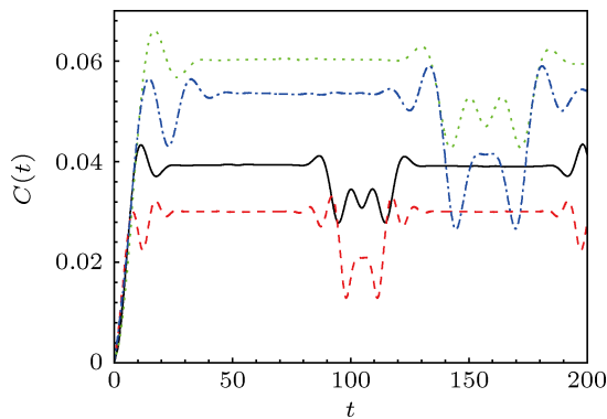
图 3 concurrence 的时间演化, 其中参数 g = 0.005, \phi = \frac{\pi}{6}: \gamma = 0.03, p = 0.5, N = 15 (实线); \gamma = 0.03, p = 0.7, N = 15 (短虚线); \gamma = 0.02, p = 0.5, N = 15 (点虚线); \gamma = 0.02, p = 0.7, N = 12 (短点虚线)
