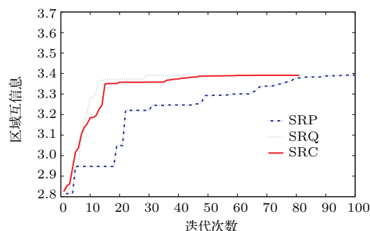
图 6 (网刊彩色) 优化过程中区域互信息随迭代次数的变化 (不同分辨率相同灰度的图像配准) Fig. 6. (color online) RMI during optimization versus number of iteration (images registration with the same gray scale but different resolutions).
