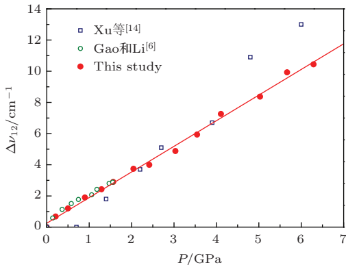
图5 (网刊彩色) 白宝石 v_{12} 不同压力下拉曼频移与前人结果对比 Fig. 5. (color online) Comparison of Raman shift of v_{12} in sapphire with previous work at different pressure.
