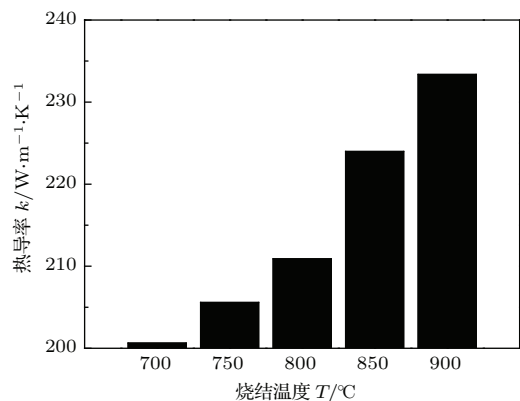
图4 热导率随烧结温度变化图 Fig. 4. Variation of thermal conductivity with the sintering-temperature.
