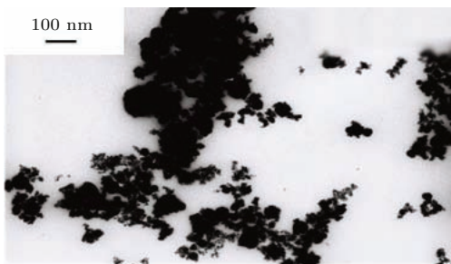
图2 纳米铜粉的TEM照片 Fig. 2. TEM micrograph of nanocrystalline Cu powder.
