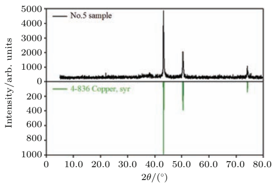
图3 纳米铜粉XRD图( 5^\circ < 2\theta < 80^\circ ) Fig. 3. X-ray diffraction pattern of Cu powders ( 5^\circ < 2\theta < 80^\circ ).
