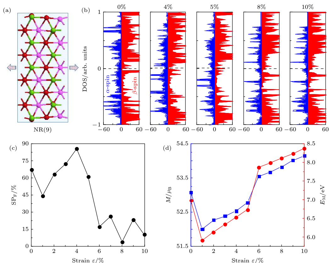
图6 应变效应 (a) 对 NR(9) 施加拉伸应力的模型图, 仅铁磁基态下被考虑; (b) 施加不同应变时的态密度 (DOS) 变化情况; (c) 费米能级上的自旋极化率 SP_F 随应变的变化; (d) 磁矩 ( M ) 和磁化能 ( E_M ) 随应变的变化 Fig. 6. Strain effects: (a) The schematic for NR(9) applied by stretching strain, only the FM ground state is taken into account; (b) the DOS versus strains; (c) the spin polarity efficiency at the Fermi level SP_F versus strains; (d) the magnetic moment ( M ) and magnetize energy ( E_M ) versus strains.
