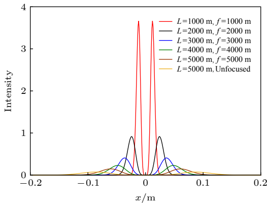
图 1 聚焦 LG 光束真空中传输不同距离的光强分布 Fig. 1. Intensity distribution of the focused LG beam propagating at different distances in vacuum.
