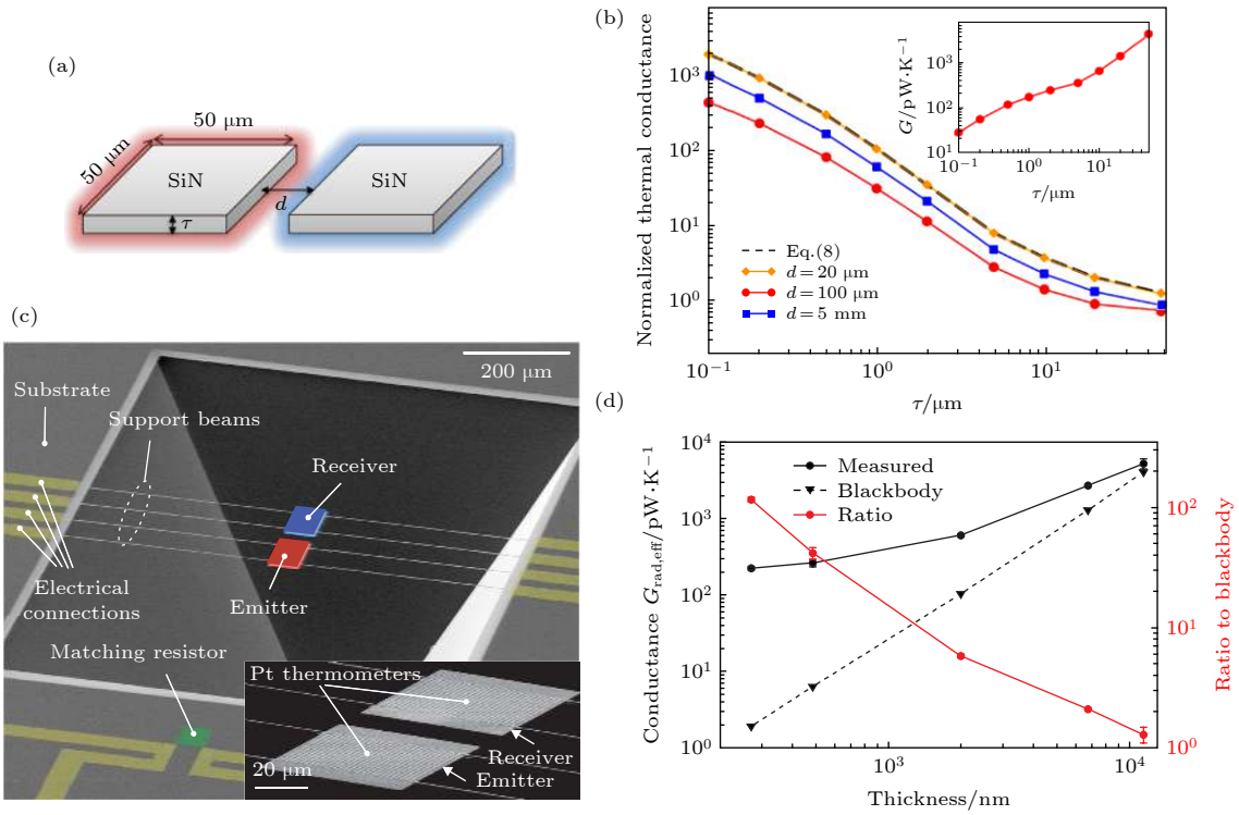
图 6 两个并列纳米平板间的远场热辐射增强示意图 (a) 和计算结果 (b) [36] ; 平行板热辐射结构 (c) 和实验结果 (d) [37] Fig. 6. Schematic (a) and theoretical simulation result (b) of enhanced far-field thermal radiation between parallel nanoplate [36] . Architecture (c) and experimental result (d) of thermal radiation between parallel plate [37] .
