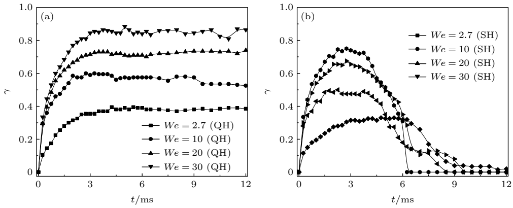
图 7 不同 We 下的动态铺展因子变化 (亲疏水分界线) (a) 液滴在 Janus 亲水侧的变化; (b) 液滴在 Janus 疏水侧的变化 Fig. 7. Dynamic spreading factor of droplet collision under different We (the hydrophilic-hydrophobic boundary): (a) Dynamic spreading factor of droplet on the hydrophilic side; (b) dynamic spreading factor of droplet on the hydrophobic side.
